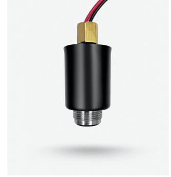
16333 3-Way DC Latching Pulse Range: 9 VDC to 24 VDC Compatible with: 3000, 3200, 3300
